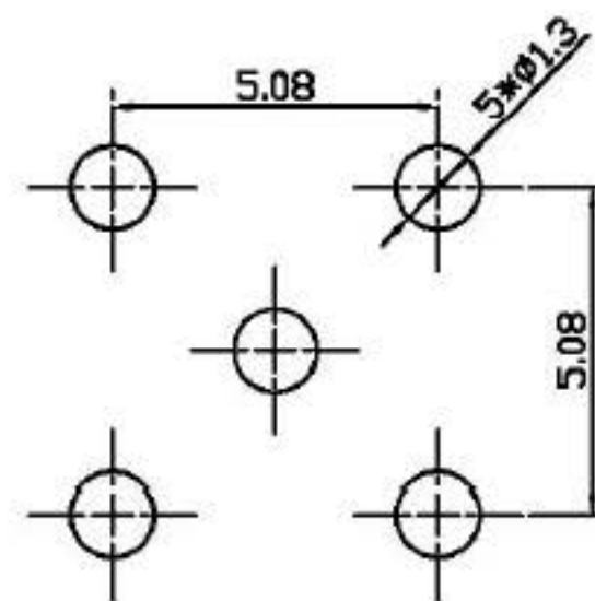
Reccmmended PCB Layout
