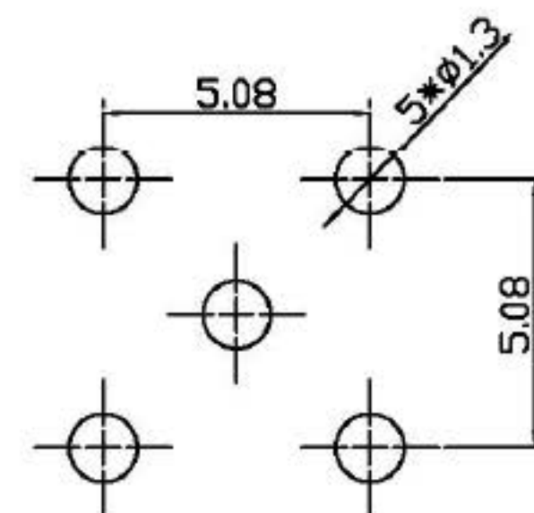
Reccmmended PCB Layout
