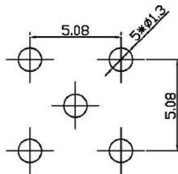
Reccmmended PCB Layout
