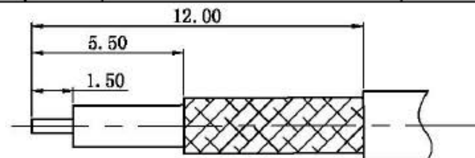
RECOMMENDED CABLE STRIPPING DIM'S (建议剥线尺寸)
