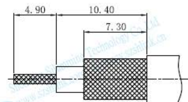
建议剥线尺寸 Recommended wire stripping size
