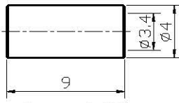
Copper tube铜管
